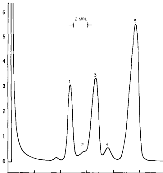
Figure 2 —Typical gas-liquid chromatogram of acetylated sample from high pH (5–8) reaction mixture. Key: Peak 1, clindamycin triacetate; Peak 2, suspected 7-epilincosamin tetraacetate or 7-epiclindamycin triacetate; Peak 3, lincomycin tetraacetate; Peak 4, unknown; Peak 5, cholesteryl acetate.
